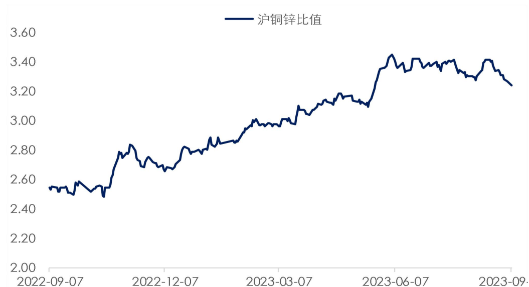
沪铜锌比值
